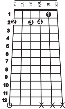
Am7/b5
